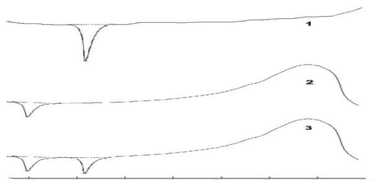
Fig.1: DSC thermograms of A) MCZ B) PEG 6000 C) F8 physical mixture
