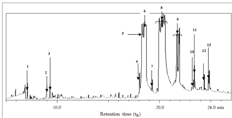
Fig. 2: Gas chromatography–mass spectrometry chromatogram of crude ethanol extract of Dacryodes edulis seed. 1 – Terpinen-4-ol (7.102 min); 2 – 5-hydroxymethylfurfural (9.006 min); 3 – 4,6,6-trimethyl Bicyclo[3.1.1]hept-3-en-2-one (9.299 min); 4 – Ethyl -9-hexadecenoate; 5 – Ethyl Hexadecanoate (18.284 min); 6 – n -hexadecanoic acid (18.527 min); 7 – 1-(+)-2,6-dihexadecanoateAscorbic acid (19.280 min); 8 – these are C18 fatty acids and their esters;9 – these are eicosanoic acids and their esters(21.929 min); 10 – Docosanoic acid (23.317); 11 – Ethyl docosanoate(23.394 min); 12 – 2,6,10,14,18-Pentamethyl-2,6,10,14,18-icopentene or squalene (24.360 min); 13 – Ethyl 14-methylhexadecanoate(24.851 min)
