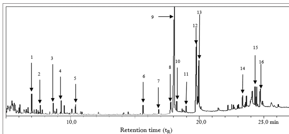
Fig. 1: Gas chromatography–mass spectrometry chromatogram of the petroleum ether crude extract of Dacryodes edulis seed. 1 – cis - p -mentha-1-(7),8-dien-2-ol (6.982 min); 2 – 2-methyl-5-(1methylethenyl)-2-cyclohexen-1-ol (7.650 min); 3 – 4- (1-methylethenyl)-2-cyclohexene-1-one (8.662 min); 4 – 4,6,6-Trimethyl bicyclo[3,1,1]-hept-3-en-2-one (9.274 min); 5–7,7-Dimethyl-3-methylenebicyclo[4.1.0]hepten-2-ol (10.384 min); 6 – Tetradecanoic acid (15.629 min); 7 – Pentadecanoic acid (16.842 min); 8 – Z -11-Hexadecenoic acid (17.774 min);9– n -Hexadecanoic acid (18.056 min); 10 – ethyl hexadecanoate (18.229 min); 11 – Eicosanoic acid (18.973 min); 12 – E -9-Octadecenoic acid (19.767 min); 13 – Octadecanoic acid (19.957 min); 14 – 2-Hydroxy-1-(hydroxymethyl) ethyl hexadecanoic acid ester (23.342 min);15 – Squalene (24.315 min); 16 – Propylene glycol monooleate (24.713 min)
