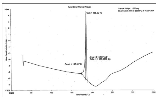
Fig. 2: Differential scanning calorimetry thermogram of paliperidone
