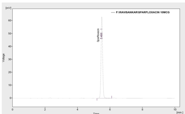
Figure3: A typical chromatogram of SPF standard
