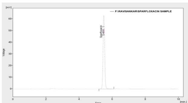
Figure 4: Chromatogram of marketed formulation (Tablets) of SPF
