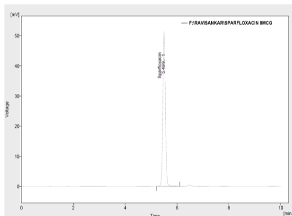
Figure 8: Standard chromatogram of SPF (8 µg/mL)
