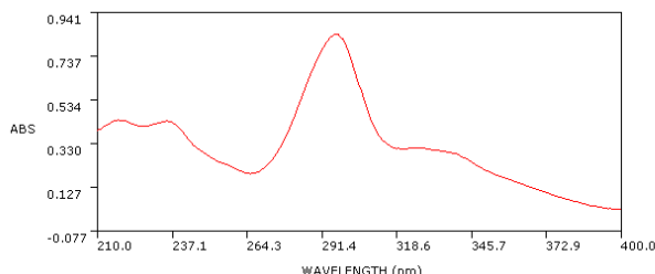
Figure 2: Absorption spectra of Sparfloxacin (291nm)
