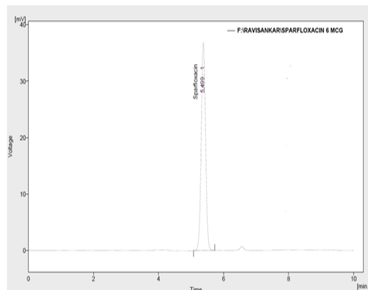
Figure 7: Standard chromatogram of SPF (6 µg/mL)
