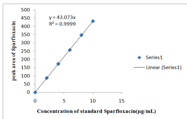
Figure 10: Calibration plot of SPF
