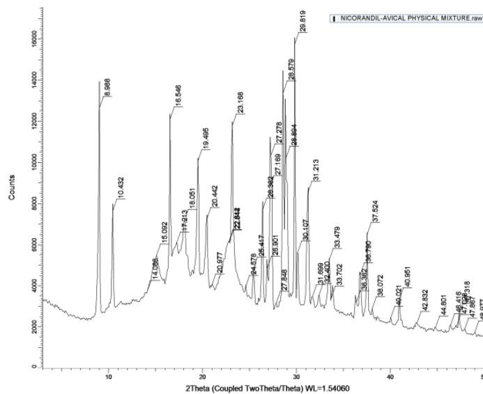
Fig. 10: PXRD patterns of nicorandi+avicel
