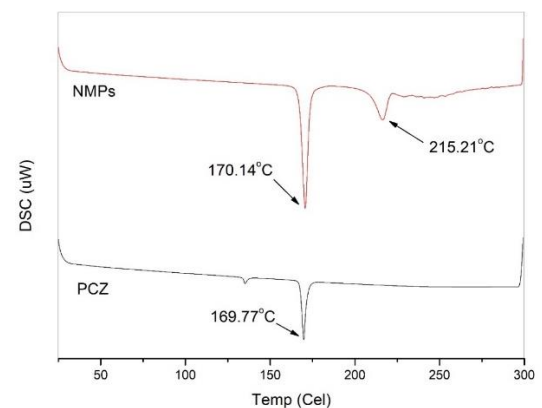
Fig. 7: DSC thermograms of posaconazole nanocrystals and the NMPs
