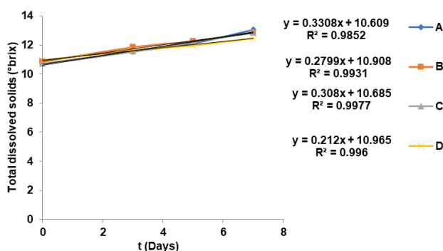
Fig. 5: Interaction of temperature and storage factors on sugarcane total dissolved solid content, A = total dissolve solid of non-sterile cane sugar at a storage temperature of 25 °C for 7 d; B = total dissolve solid of sterile cane juice at a storage temperature of 25 °C for 7 d; C = total dissolve solid of non-sterile cane juice at a storage temperature of 5 °C for 7 d; D = total dissolve solid of sterile cane juice at a storage temperature of 5 °C for 7 d
