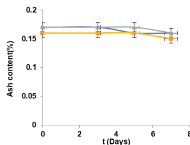
Fig. 3: Interaction of temperature and storage factors on ash content sugarcane, A = ash content non-sterile cane sugar at a storage temperature of 25 °C for 7 d; B = ash content of sterile cane juice at a storage temperature of 25 °C for 7 d; C = ash content of non-sterile cane juice at a storage temperature of 5 °C for 7 d; D = ash content of sterile cane juice at a storage temperature of 5 °C for 7 d
