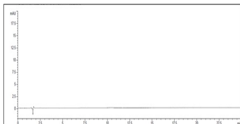
Fig. 2: Chromatogram of placebo solution of Nadifloxacin
