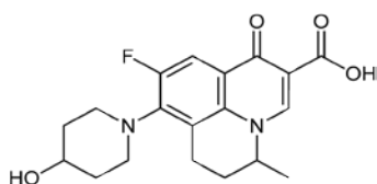
Fig. 1: Structure of Nadifloxacin
