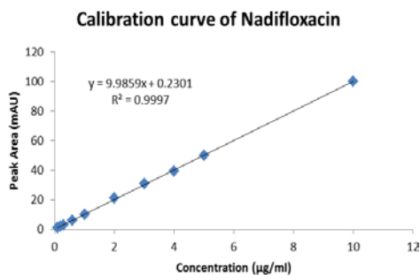
Fig. 4: Calibration curve of Nadifloxacin
