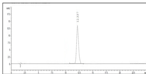
Fig. 3: Chromatogram of Nadifloxacin
