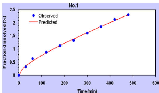
Fig. 11: predicted and observed value of optimised formulation (F3)
