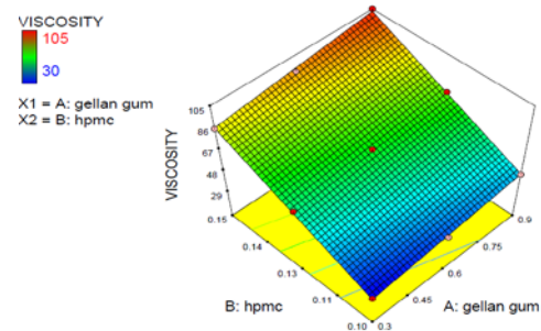
Fig. 4: Anova result for viscosity
