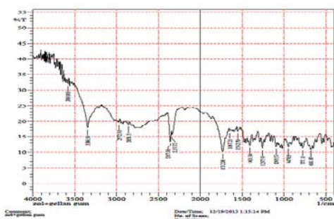
Fig. 3: FTIR spectra of plane of drug Zolmitriptan
