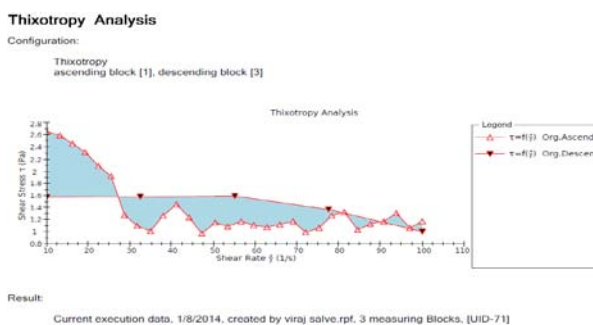
Fig. 8: Thixotropy analysis study of optimised formulation (F3)
