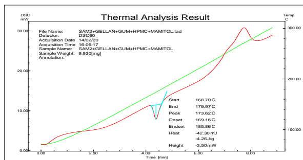
Fig. 5: DSC graph for mixture of polymer and drug
