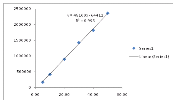
Fig. 4: Linearity graph for ATV
