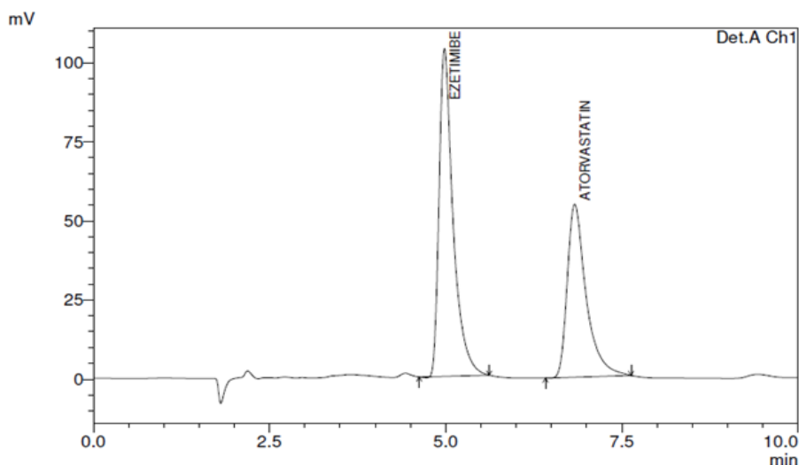
Fig. 8: Assay of Statix-Ez®
