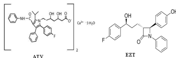
Fig. 1: Chemical structures of atorvastatin calcium and Ezetimibe
