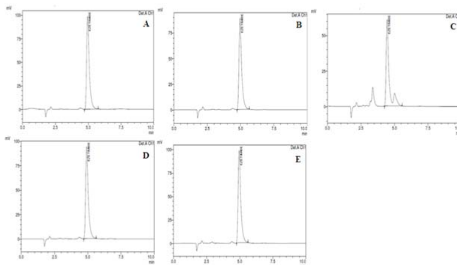
Fig. 7: Typical degradation chromatograms of EZT; A) Control sample; B) 0.1 N HCL at 25 °C after 24 h; C) 0.1 N NaOH at 25 °C after 24 h; D) 3 % H 2 O 2 at 25 °C after 24 h; E) UV light (210 nm) after 24 h
