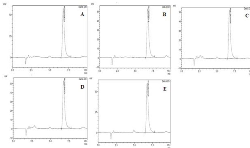
Fig. 6: Typical degradation chromatograms of ATV; A) Control sample; B) 0.1 N HCL at 25 °C after 24 h; C) 0.1 N NaOH at 25 °C after 24 h; D) 3 % H 2 O 2 at 25 °C after 24 h; E) UV light (210 nm) after 24 h
