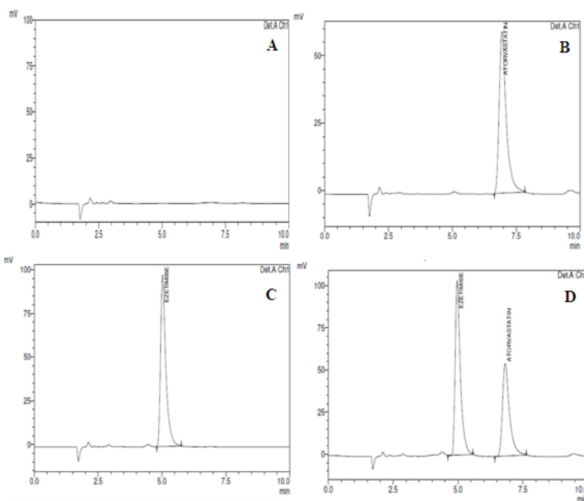
Fig. 2: Typical specificity chromatograms: A) blank sample: B) EZT: C) ATV: D) Both ATV and EZT
