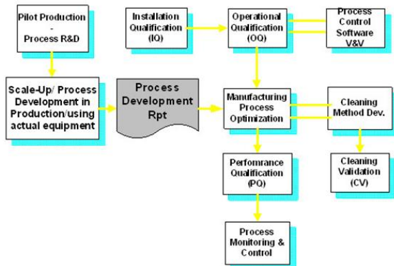
Fig.4: Manufacturing Process Validation Workflow [4]
